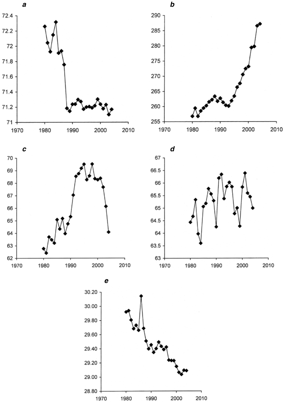
Figure 1 — Change in overall tour performance on (a) scoring average, (b) driving distance, (c) driving accuracy, (d) greens in regulation, (e) and putts per round over time for the selected sample of golfers.
