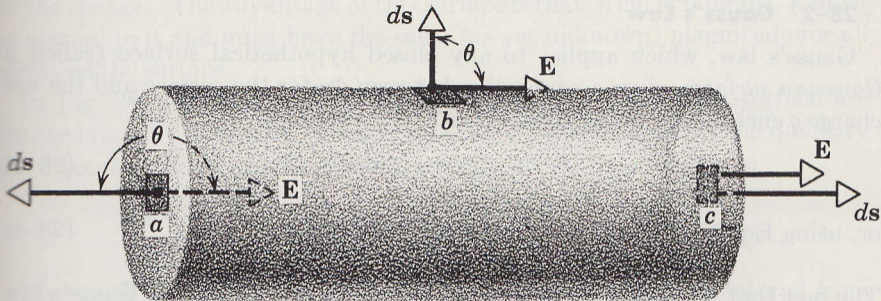
Fig. 28-3 Example 1. A cylindrical surface immersed in a uniform field \mathbf{E} parallel to its axis.
