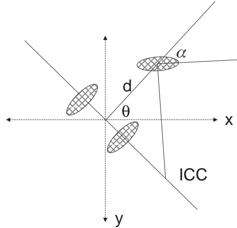
Figure 2. Bicycle/tricycle kinematics. The shaded ovals represent the three wheels of Trike . The instantaneous centre of curvature (ICC) must lie at the intersection of lines orthogonal to, and passing through the rotation axis of each wheel.
