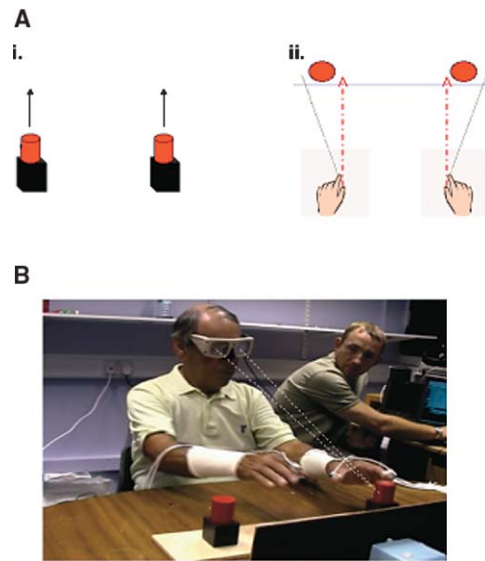
Figure 2. Task Characteristics
