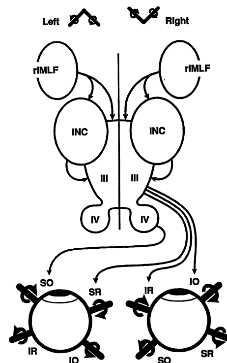
Fig. 1. Schematic diagram of the midbrain structures involved in generating vertical and torsional saccades. Brain structures and eyes are viewed from above the subject. Only excitatory connections are illustrated. During a saccade, neurons in the rostral interstitial nucleus of the medial longitudinal fasciculus (riMLF) send a burst of activity directly to ipsilateral motoneurons of the third and fourth cranial nerve nuclei and to the ipsilateral INC. The current investigation suggests that the INC converts this burst into a position signal, which tonically excites the ipsilateral motoneurons. Motoneurons of the right brain innervate eye muscles that rotate the eyes clockwise and vertically, whereas motoneurons of the left brain innervate the counterclockwise-vertical muscles. Thick lines projecting from the eyes show the axes and direction of rotation produced by the individual muscles. The small axes at the top of the figure summarize the rotations controlled by neurons on each side. III, oculomotor nucleus; IV, trochlear nucleus; SO, superior oblique muscle; SR, superior rectus; IR, inferior rectus; IO, inferior oblique.
