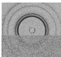
X-rays diffracted by a metal foil
