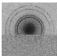
Electrons diffracted by a metal foil
