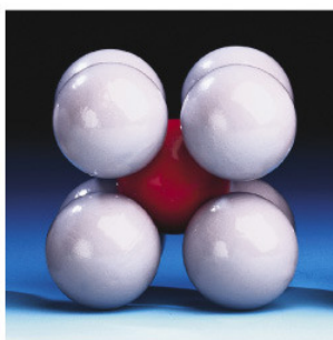
Body-centered cubic
