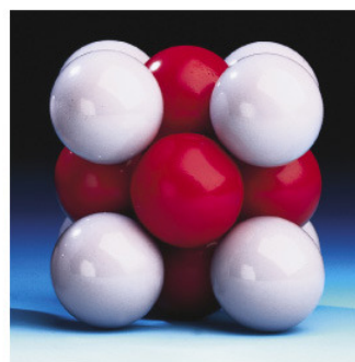
Face-centered cubic
