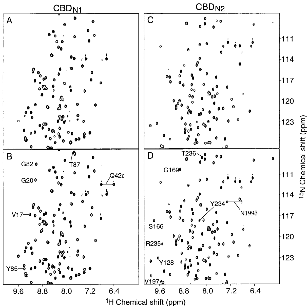
Figure 3. Portions of the non-sensitivity enhanced ^1\text{H} - ^{15}\text{N} HSQC spectra of (a), (b) \text{CBD}_{\text{N1}} and (c), (d) \text{CBD}_{\text{N2}} bound to (a), (c) oxidized or (b), (d) reduced TEMPO-Glc 4 . The final ligand-to-protein ratios of 2.2:1 and 1.4:1 correspond to \sim 80\% and 65\% saturation of \text{CBD}_{\text{N1}} and \text{CBD}_{\text{N2}} , respectively. Peaks from amides that “disappear” because of paramagnetic relaxation due to the nearby unpaired electron in the nitroxide-labeled cellotetraose are identified.
