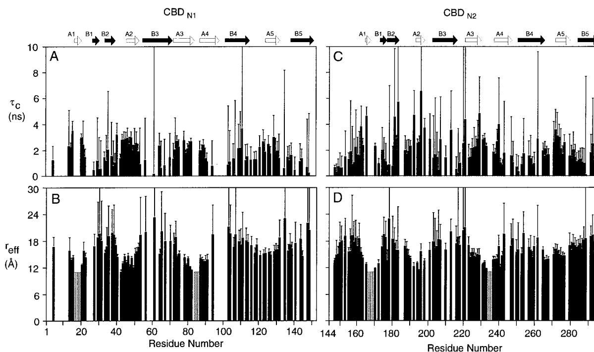
Figure 6. The correlation times, \tau_c , and effective electron-proton distances, r_{eff} , calculated for (a), (b) CBD N1 and (c), (d) CBD N2 bound to TEMPO-Glc 4 . Residues whose signals disappear completely due to severe linebroadening are shown with a shaded bar at an upper bounds of r_{eff} = 11 Å. The locations of the \beta -strands forming sheets A and B in the two proteins are indicated by the open and filled arrows, respectively.
