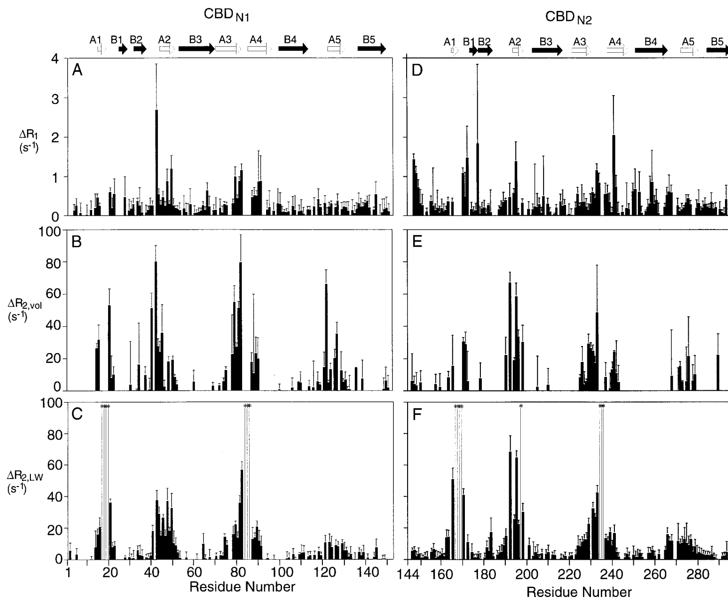
Figure 4. The enhancement of the amide ^1\text{H}^{\text{N}} longitudinal ( \Delta R_1 ) and transverse ( \Delta R_{2,\text{vol}} and \Delta R_{2,\text{LW}} ) rates resulting from the binding of TEMPO-Glc 4 by (a), (b), (c) CBD N1 and (d), (e), (f) CBD N2 . Only positive rate enhancements are shown. Residues whose signals disappear completely due to the nitroxide spin label are identified in (c) and (f) with an asterisk. The locations of the \beta -strands forming sheets A and B in the two proteins are indicated by the open and filled arrows, respectively.
