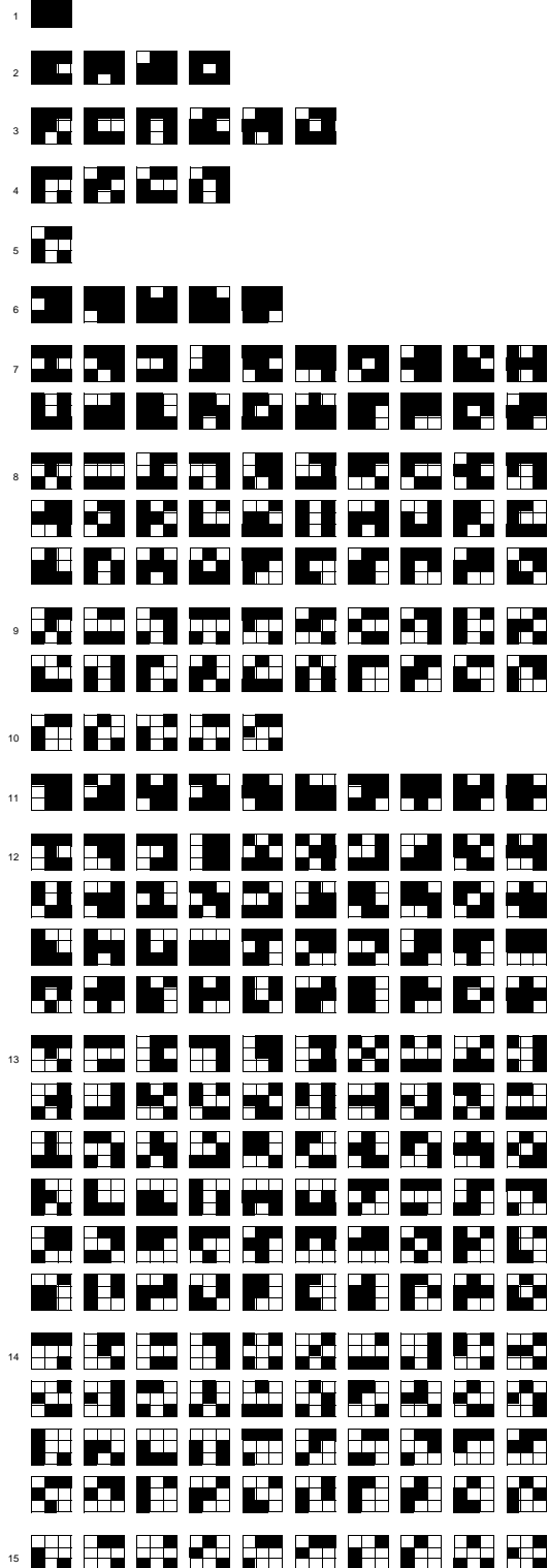
Supplementary Figure All possible maps given the coincidence matrices in Figure 3, given map A provided at the top-left corner of this figure. The numbers refer to the unique coincidence matrix identifiers.
