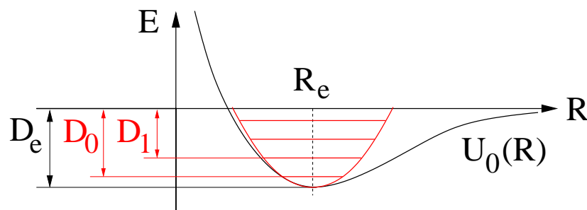
Figure 5.2: Typical ground-state PES and harmonic oscillator model of vibrational motion. D_e = U_0(R_e) is the binding energy and D_0 = D_e - \frac{\hbar\omega_e}{2} the dissociation energy of the molecule.
