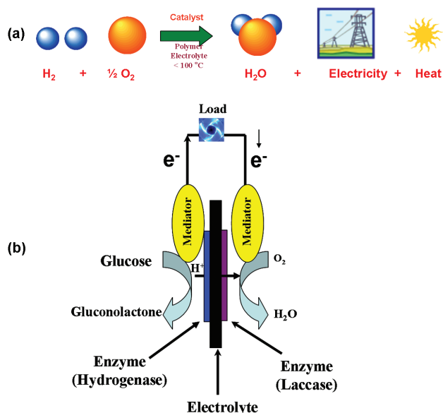
Fig. 1. (a) Principle of a low temperature \text{H}_2/\text{O}_2 fuel cell, (b) operating principle of a biofuel cell involving hydrogenase and laccase enzymes.
