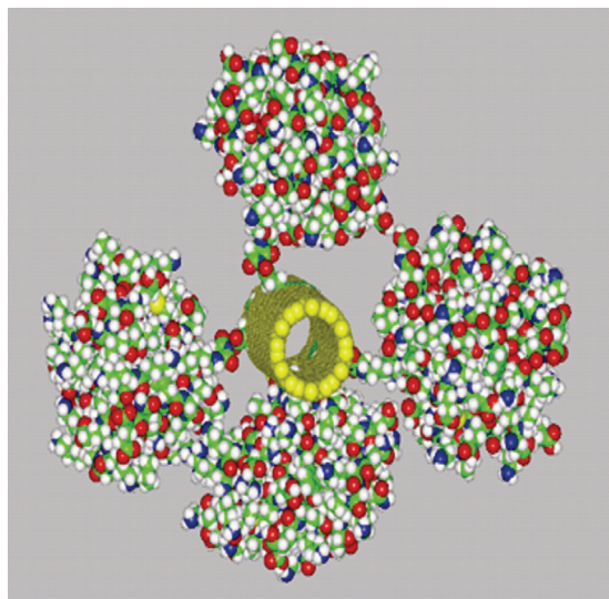
Fig. 13. Molecular dynamics simulation of GOx with SWCNT. Reprinted with permission from [40], S. S. Tatke et al., Nanotechnology 15, S684 (2004). © 2004, IOP Publishing Ltd.
