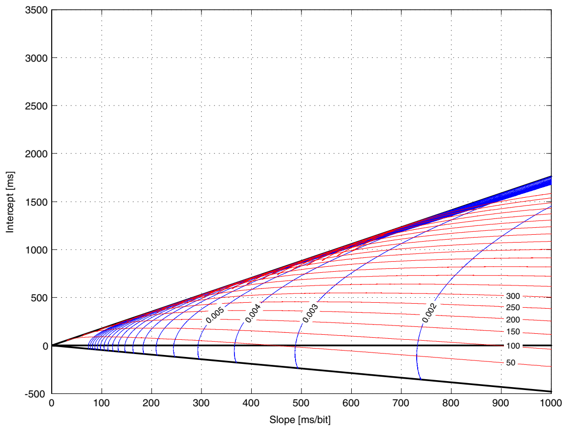
Fig. 8 Contour diagram of the relationship between the linear regression slope and Y -intercept, and the model parameters, delay \tau (red) and DV population relaxation rate \alpha (blue) using the movement-based definition of movement time. Contours for delay are every 50 ms.
