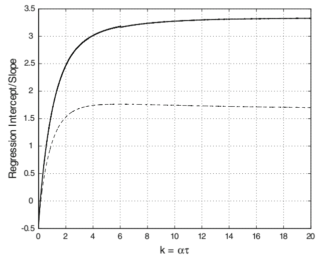
Fig. 3 Graph of the intercept divided by slope for linear regression of the performance curve MT_{1,k}(ID) as a function of k . The solid line uses the stimulus-based definition of MT while the broken line uses the movement-based definition. Regression curves are computed by sampling the performance curve at intervals of 0.2 bits between 1 and 10 bits
