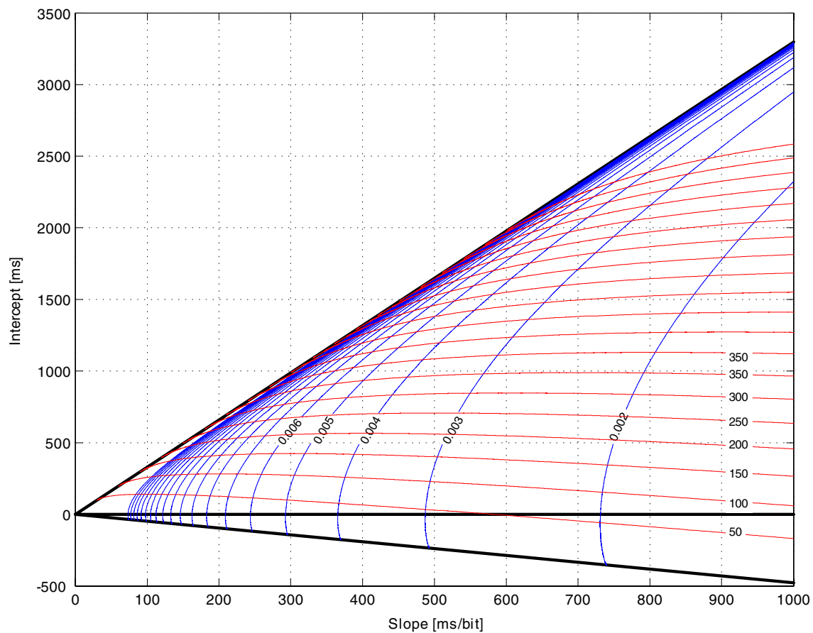
Fig. 6 Contour diagram of the relationship between the Fitts' law slope and Y-intercept, and the model parameters, delay \tau (red) and DV population relaxation rate \alpha (blue) using the stimulus-based definition of move-
