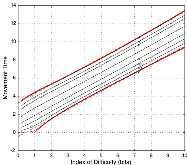
Fig. 2 Performance curves MT_{1,k}(ID) are normalized so that the linear regression has a slope of 1 ( solid ) and the regression line ( dotted ) for k = \alpha\tau of 0, 0.01, 0.1, 0.25, 0.5, 1, 2, 3, 10, and \infty . Observe that these curves approach a limit as k \rightarrow 0 or k \rightarrow \infty . The normalized performance curves as k = \alpha\tau \rightarrow 0, \infty are shown in red . The only possible performance curves for the delayed feedback circuit are the constant multiples of these, and thus only take on a finite range of slope and intercept values (color figure online)
