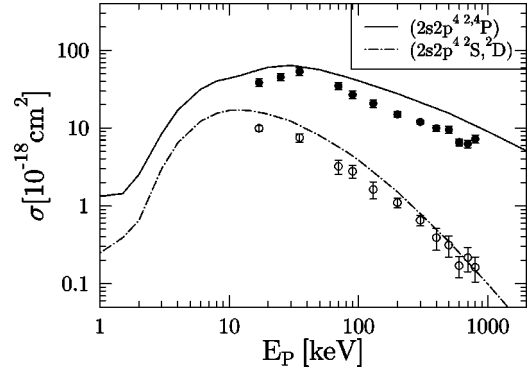
FIG. 10. Total cross sections for transitions to the final states O^+(2s2p^4\ ^{2,4}P) and O^+(2s2p^4\ ^2S, ^2D) as a function of impact energy for p -O collisions. Theory: present calculation with OPM potential and analysis in terms of particle-hole probabilities [Eq. (25)] as described in the text. Experiment: fluorescence emission cross sections for (●) O^+(2s2p^4\ ^{2,4}P) final states and (○) O^+(2s2p^4\ ^2S, ^2D) final states [18].
