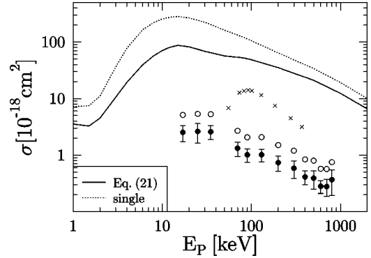
FIG. 9. Total cross sections for excitation of the final state O(2s 2p^5 ^3P) as a function of impact energy for p -O collisions. Theory: present calculation with OPM potential and analysis in terms of determinants [Eq. (21)], and single-particle cross section for 2s \rightarrow 2p excitation (single); Experiment: (●) fluorescence emission cross sections [18]; (○) fluorescence data corrected for autoionization as described in the text; (×) excitation cross sections for e -O collisions [27].
