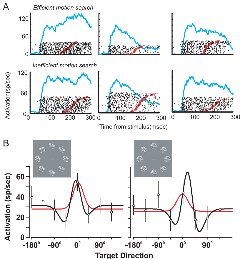
FIG. 3. Activity of the same neuron during motion search. Same conventions as Fig. 2. Parameters of the difference-of-Gaussian function for efficient search were B = 81 sp/s, R_+ = 54 sp/s, \Phi_+ = -5^\circ , and T_+ = 2^\circ , R_- = 31 sp/s, \Phi_- = -11^\circ , and T_- = 39^\circ . The parameters for less efficient search were B = 77 sp/s, R_+ = 39 sp/s, \Phi_+ = 12^\circ , T_+ = 20^\circ , R_- = 22 sp/s, \Phi_- = -26^\circ , T_- = 44^\circ .
