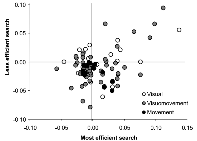
FIG. 4. Difference between the Model Selection Criterion (MSC) values for difference-of-Gaussian and single Gaussian fits for less efficient search plotted against the difference for efficient search for visual neurons (open symbols), visuomovement neurons (gray symbols), and movement neurons (closed symbols). Values > 0 were categorized as exhibiting significant suppressive surrounds.
