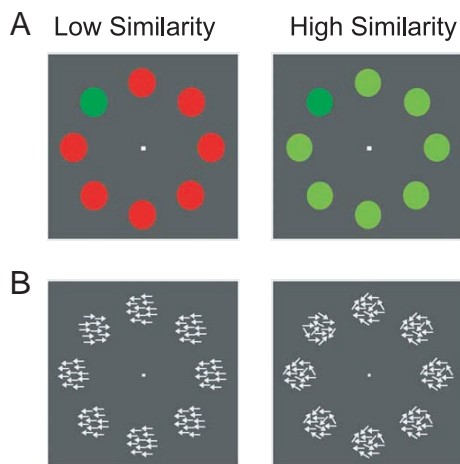
FIG. 1. Visual displays requiring localization of a singleton defined by color (A) or motion (B) with stimuli that support efficient (left) and inefficient (right) search. Efficient and inefficient displays were interleaved. Color and motion search was blocked.
