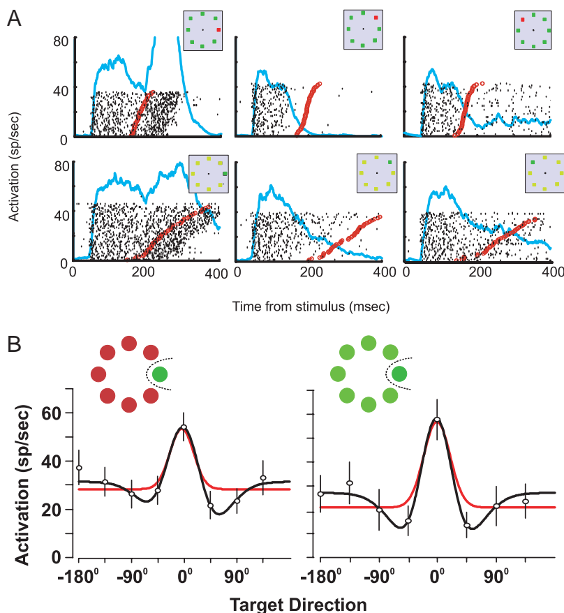
FIG. 2. Activity of a frontal eye field (FEF) neuron during color search. A: activity during interleaved efficient (top) and less efficient (bottom) search. In the raster displays, vertical tickmarks represent times of neuronal discharges. Rasters are aligned on target presentation and sorted according to interval between target presentation and saccade initiation. Superimposed on the raster is the average spike density function. Saccade initiation is indicated by the solid circle in each raster line. Inset: configuration of stimuli to which the monkey was responding. Shaded region indicates extent of receptive field. Activation was greatest when the target fell in the receptive field (left). Note the stronger, more rapid suppression of the response to the distractor when the target was beside the receptive field (middle) compared with when it was distant (right). B: selective response to stimulus in receptive field as a function of direction of the target during efficient (left) or inefficient (right) search. By convention, 0^\circ corresponds to the center of the receptive field; positive angles progress counterclockwise, and negative angles, clockwise. Vertical lines indicate 1 SE. Parameters of the difference-of-Gaussian function for efficient search were B = 31 sp/s, R_+ = 48 sp/s, \Phi_+ = -2^\circ , and T_+ = 26^\circ , R_- = 26 sp/s, \Phi_- = -6^\circ , and T_- = 52^\circ and for inefficient search were B = 27 sp/s, R_+ = 66 sp/s, \Phi_+ = -1^\circ , T_+ = 23^\circ , R_- = 36 sp/s, \Phi_- = 0^\circ , T_- = 48^\circ .
