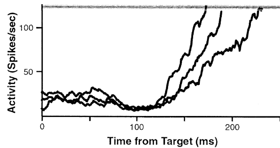
Figure 4. Relationship between Movement-Related FEF Activity and Saccade Initiation
