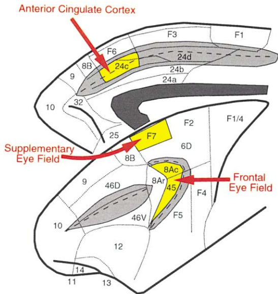
Figure 1. Anatomical Subdivisions of Macaque Frontal Cortex The dorsolateral (lower) and mesial (upper) surface of the frontal lobe are shown. The location of the frontal eye field (areas 8Ac and 45), supplementary eye field (area F7), and the portion of anterior cingulate cortex connected with the supplementary eye field (in area 24c) are highlighted in yellow. Gray areas represent opened sulci, showing the fundus as a dashed line. Boundaries between labeled areas are indicated by dotted lines.
