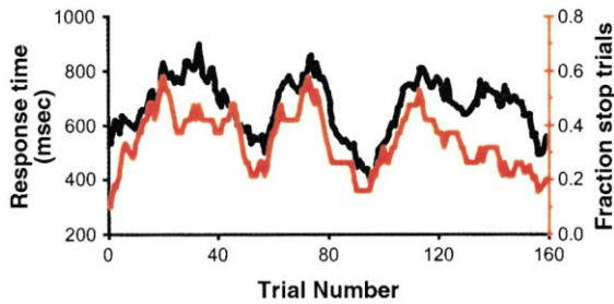
Figure 3. Covariation of the Running Average of Response Time of Monkeys on Trials with No Stop Signal (Black) and the Running Average of the Fraction of Stop Signal Trials (Red)
